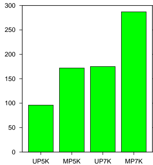
Figure 14: Developer Performance
